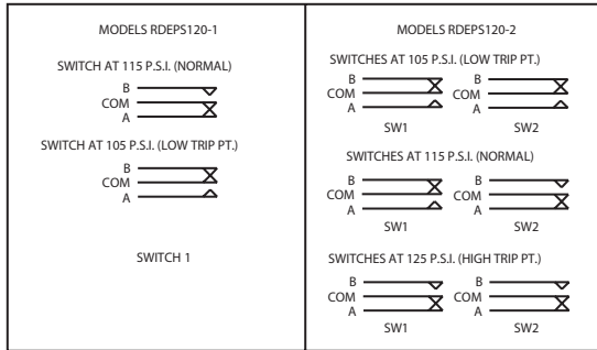
Figure 3. Electrical Connections
